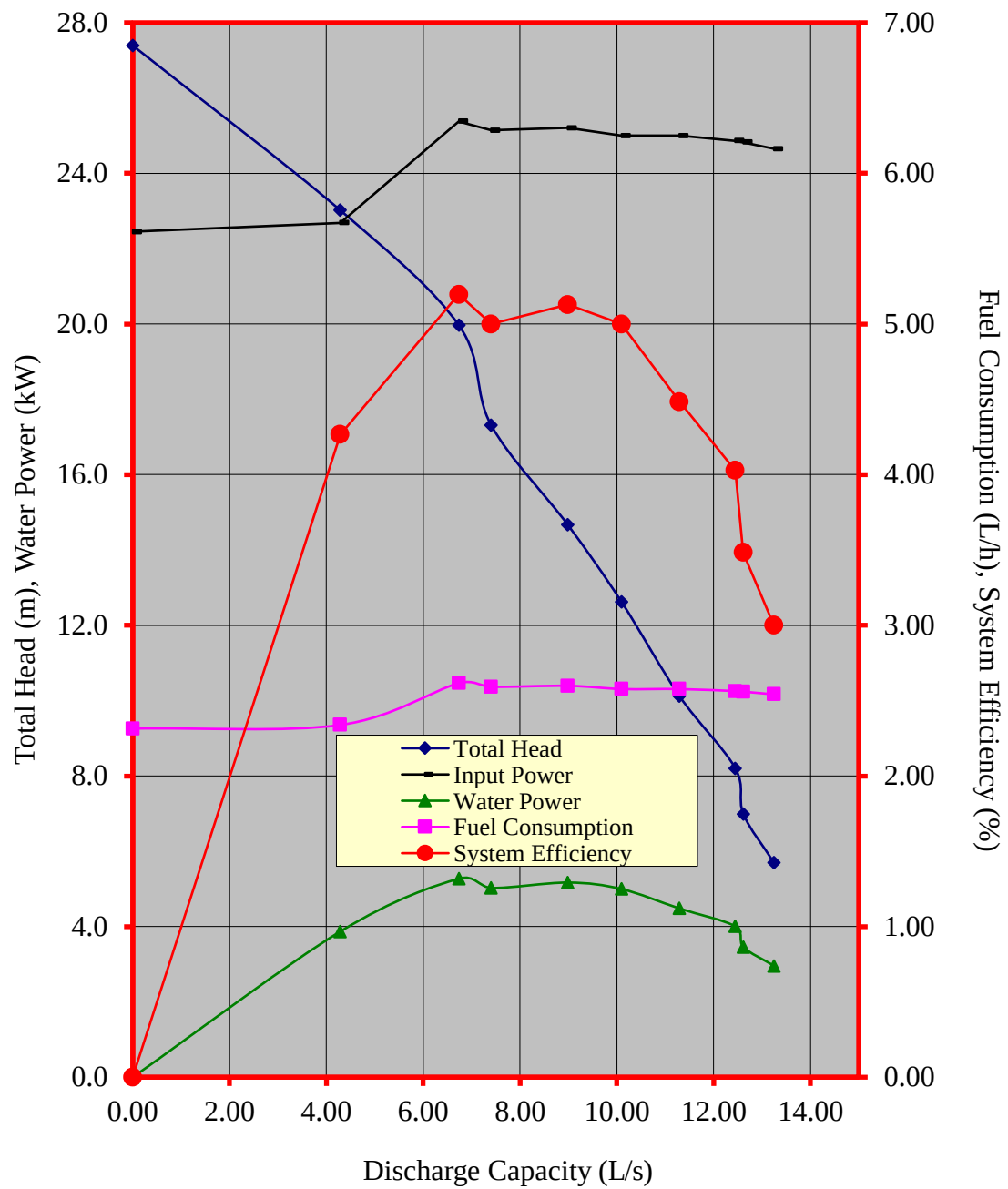
Figure 3. Performance characteristic curves of the PLATINUM PT6.5 HP self-priming centrifugal pumpset
